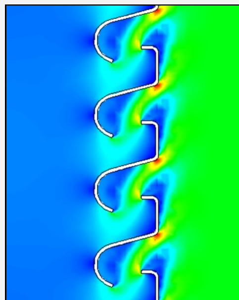
EFD simulation
